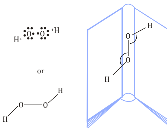
Open book like structure of \text{H}_2\text{O}_2
