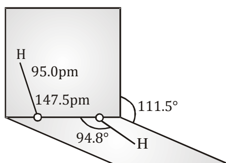
(a) Gas phase
